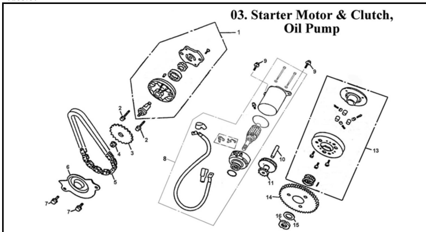
Starter Motor, Starter Clutch and Oip Pump
