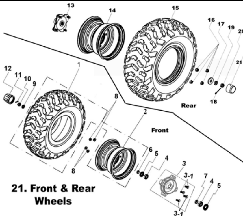
Front and Rear Tires and Wheels
