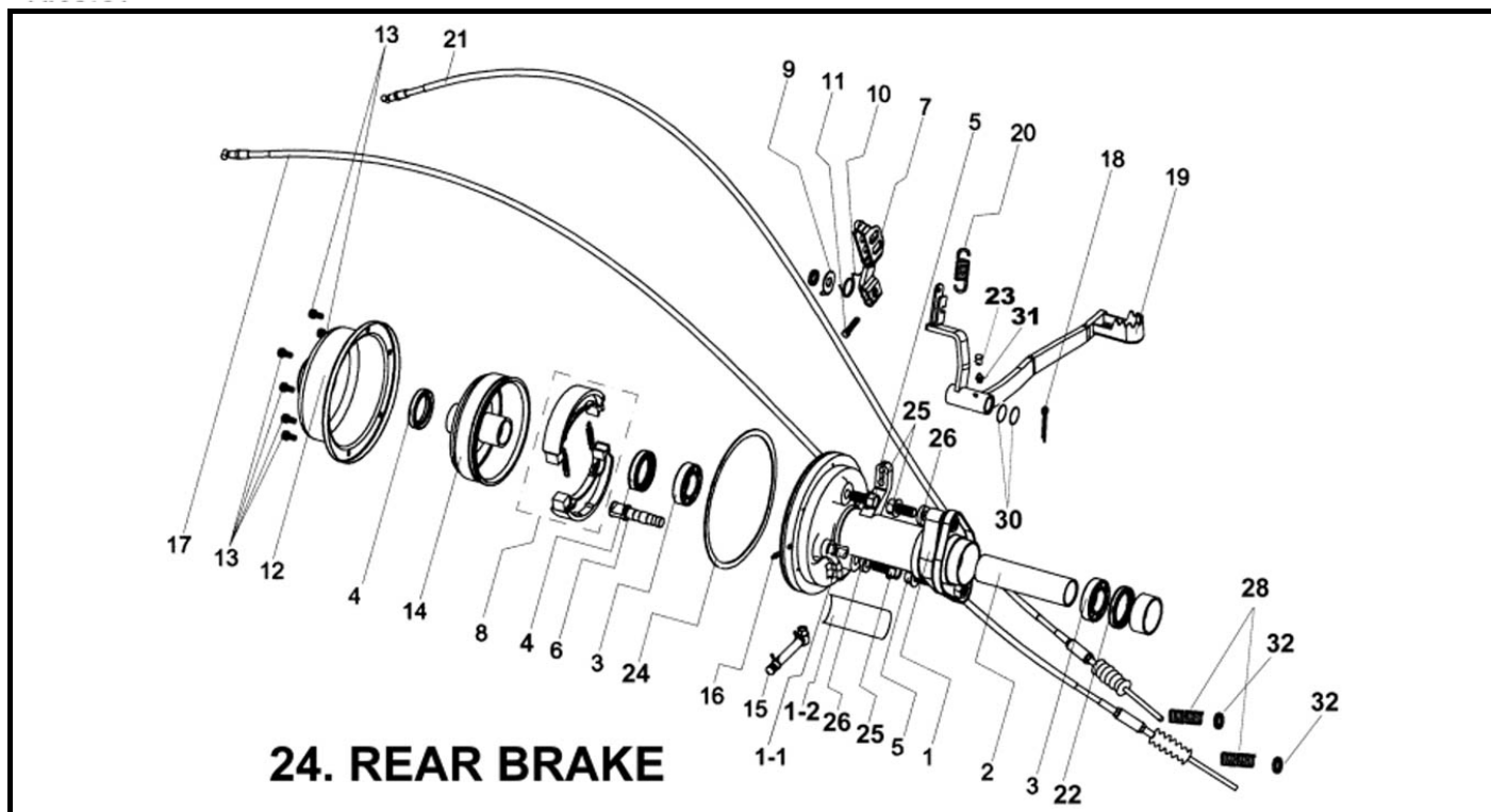
Rear Brake
