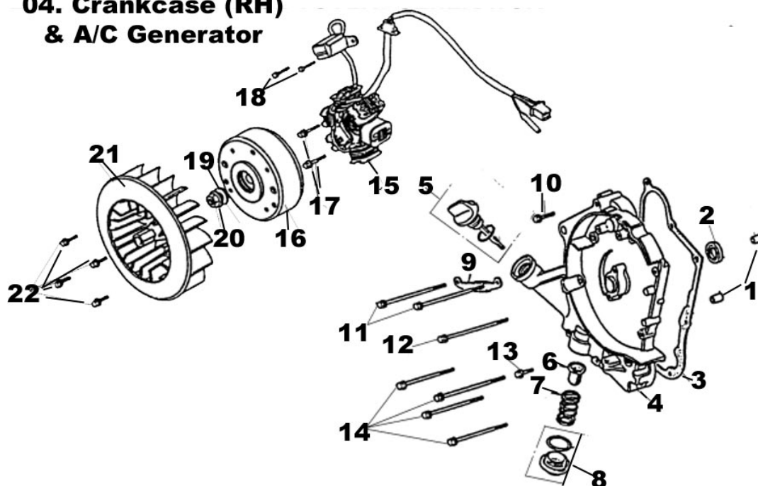
Crankcase (RH) and A/C Generator
