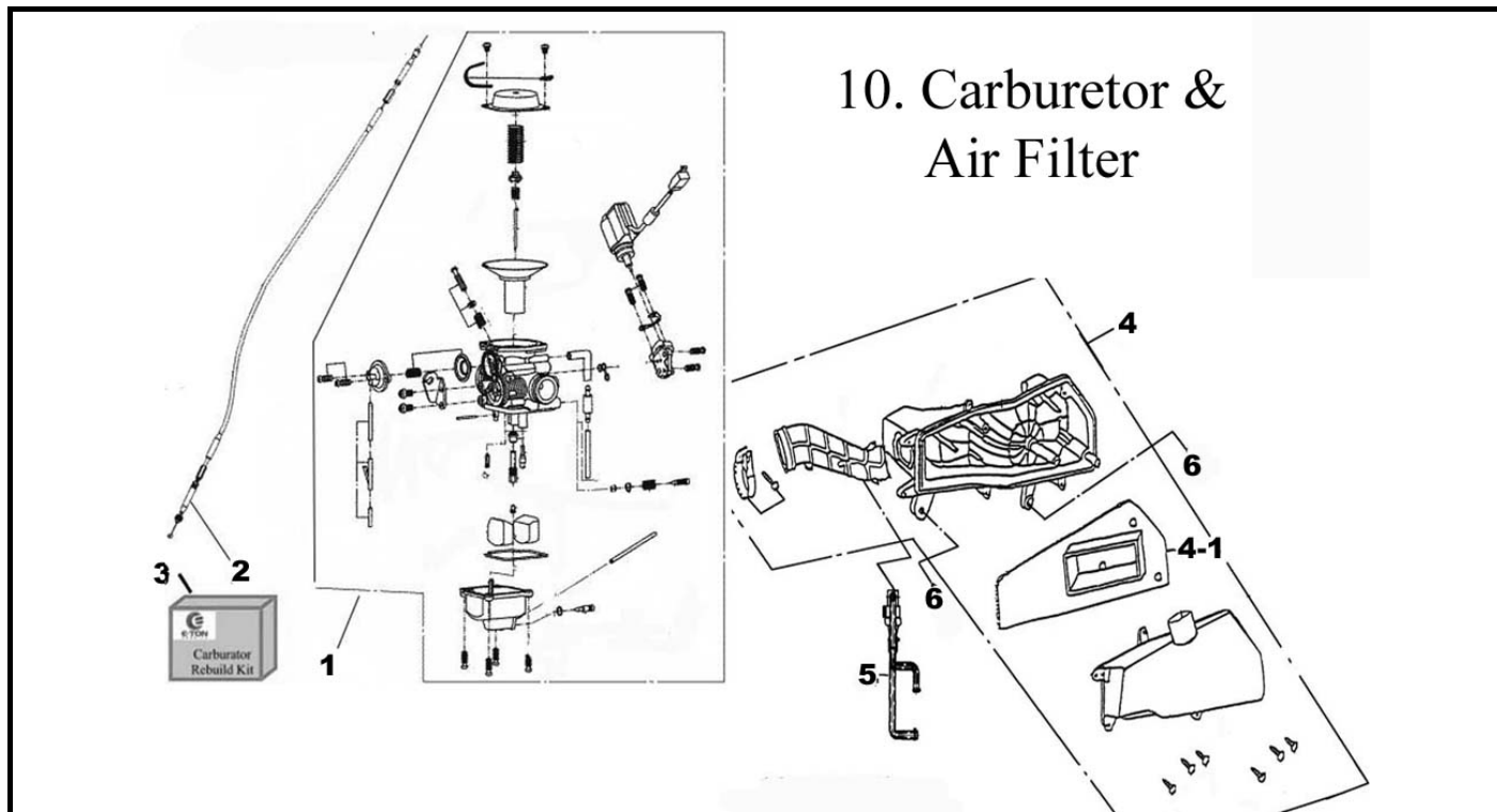
Carburetor, Throttle Cable and Air Filter
