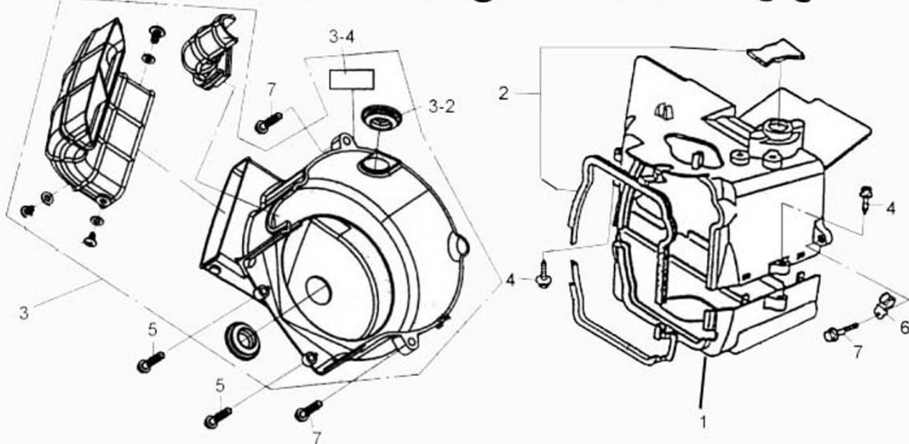
Fan Cover and Engine Shroud
