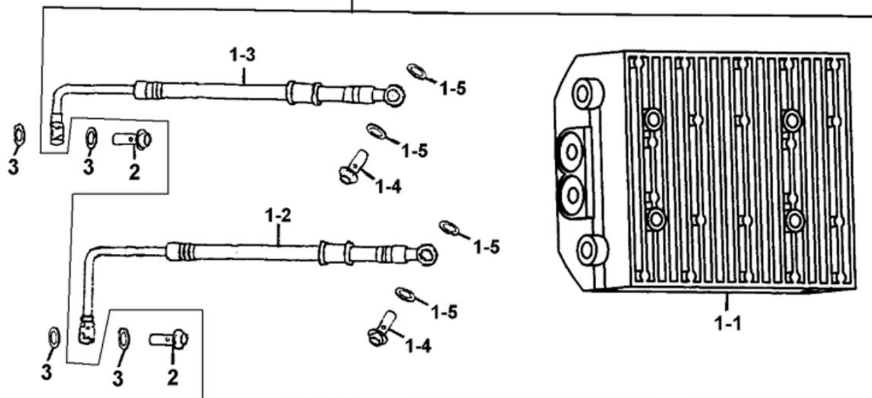
Engine Oil Cooler
