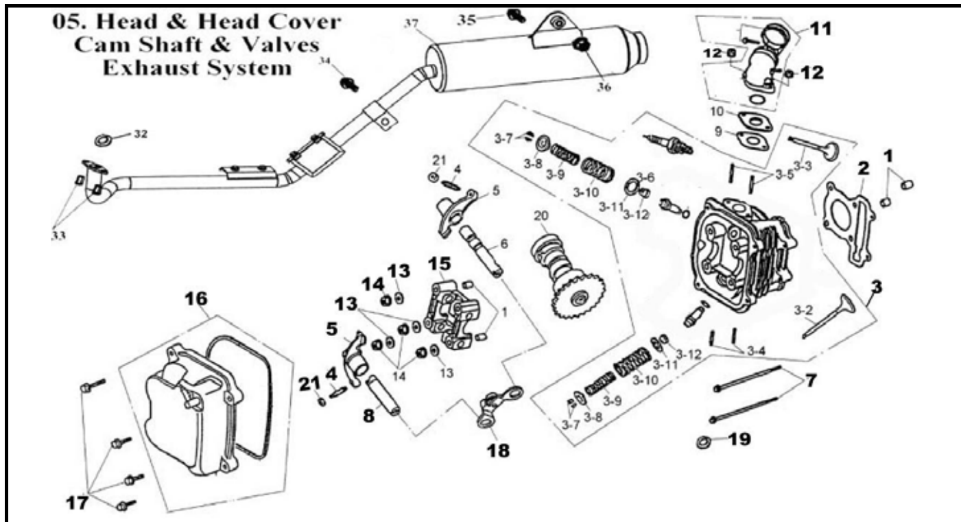
Head, Head Cover, Camshaft, Valves and Exhaust
