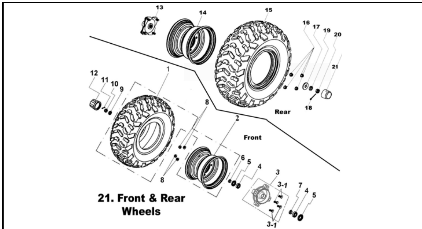
Front and Rear Tires and Wheels
