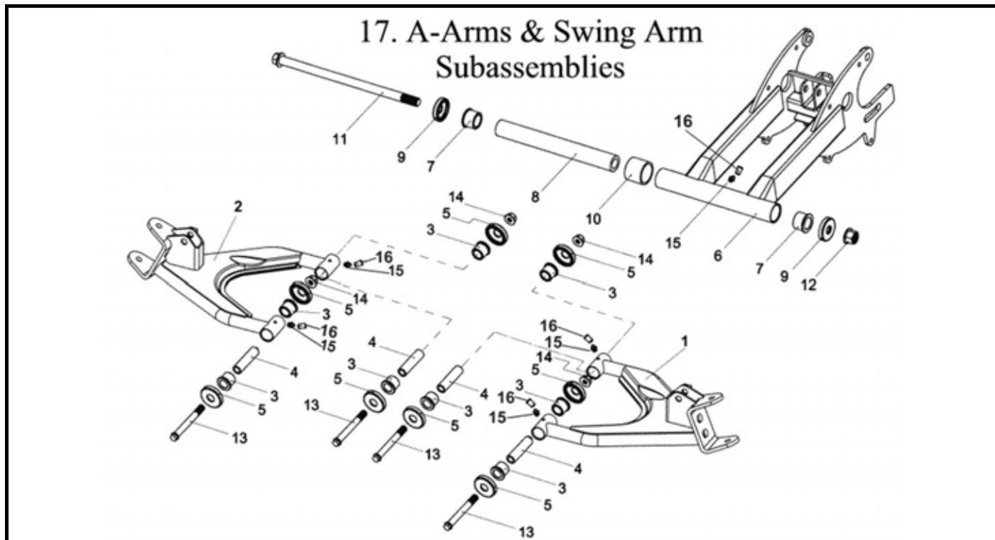
A-Arms and Swing Arm
