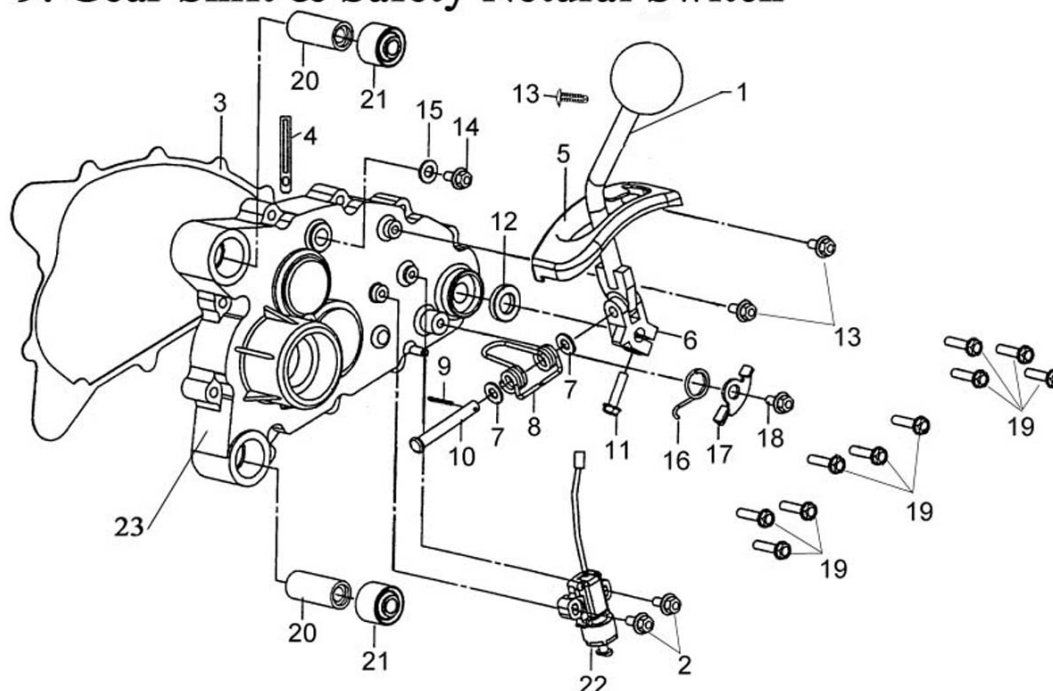
Gear Shift and Safety Netrul Switch
