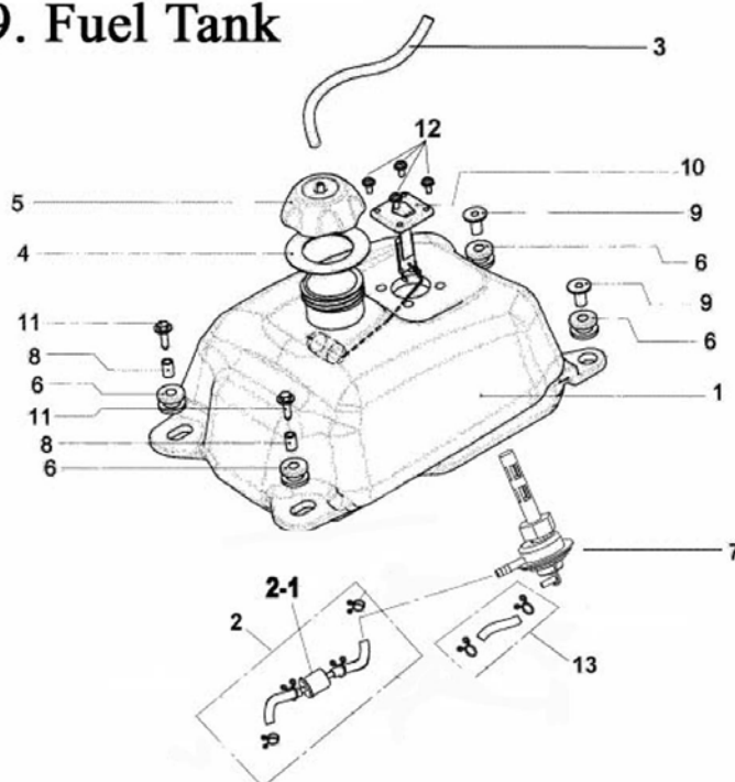
Fuel Tank
