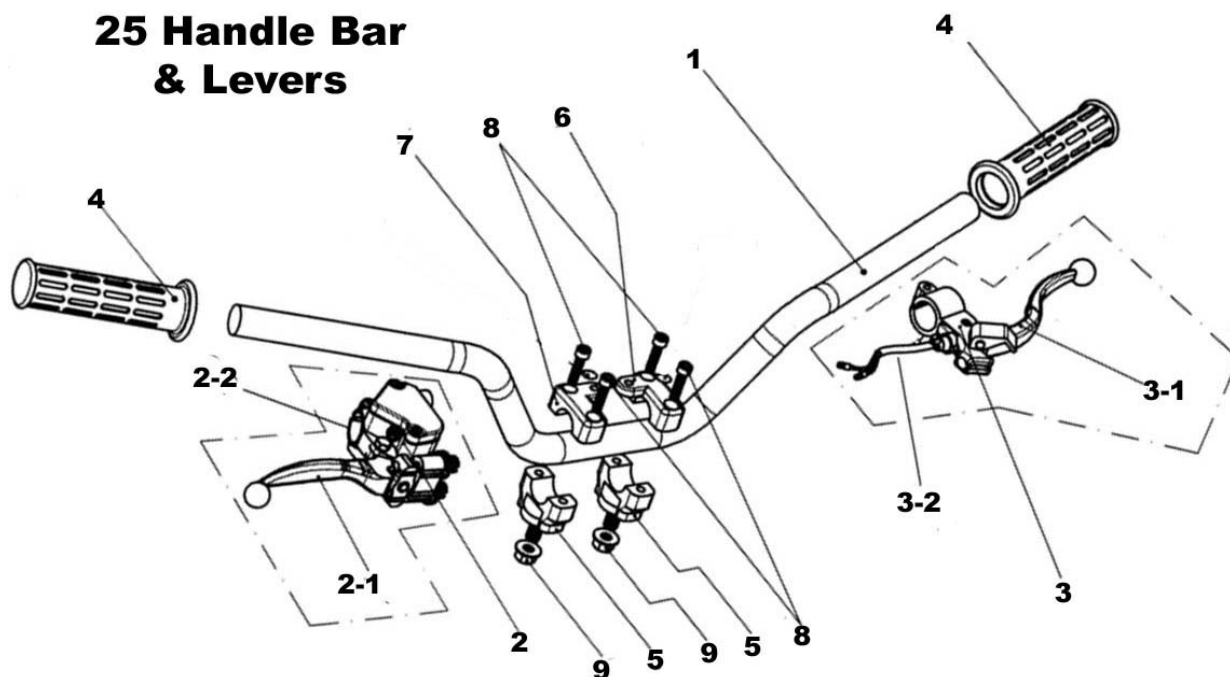
Handle Bar and Levers
